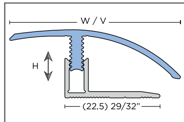
Reducer TP1-
