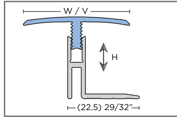
Transition TP3-
